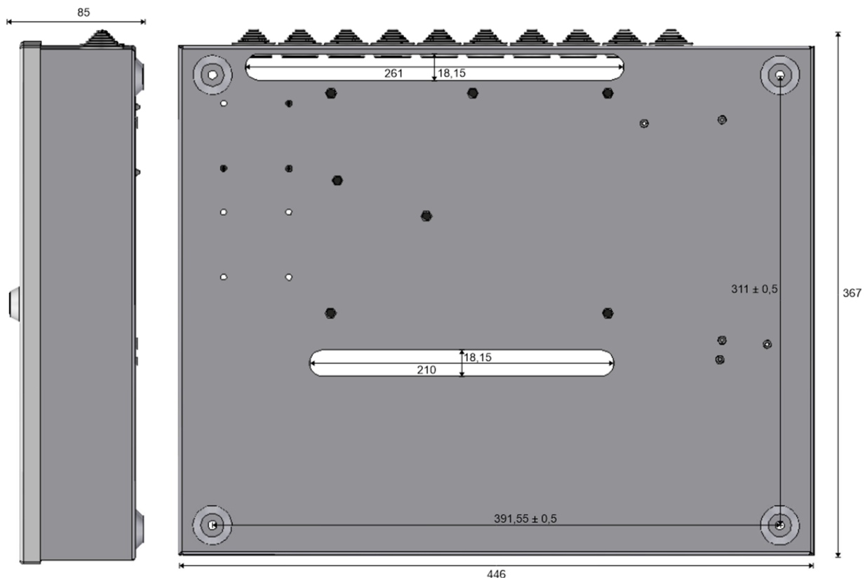
Dimensional drawing (mm):
